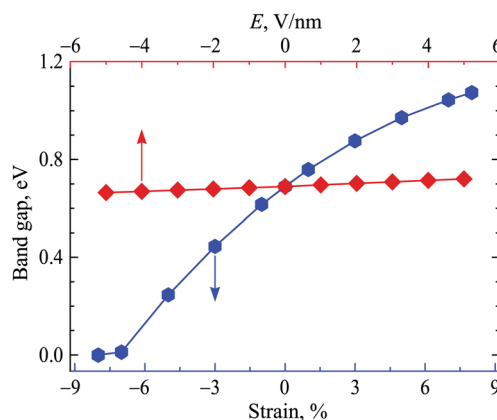
Fig. 8 Dependence of band gap of Janus ZrSSe on strain engineering and electric field E .
